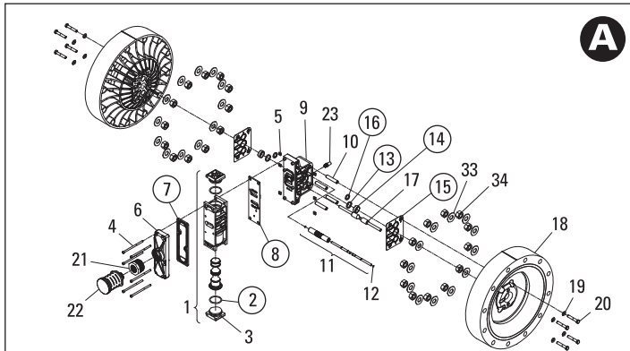
PLASTIC ADS
